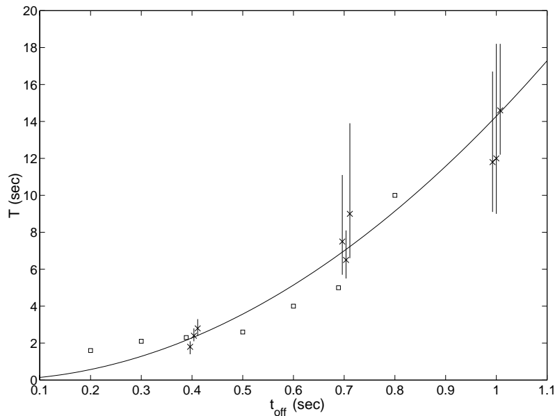
Figure 4: Mean dwell time T as a function of the off-time t_0 in discontinuous presentation. The solid curve is a one-parameter fit (leading to \Delta t = 70 ms) from the prediction of the Necker-Zeno model under the assumption that the off-time can be identified with the decay time t_0 of the unperturbed system.
