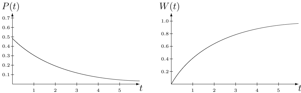
Figure 5: The probability density P(t) (left) for a switch of the mental state at time t and the cumulative probability W(t) (right) that a switch occurred up to time t .
