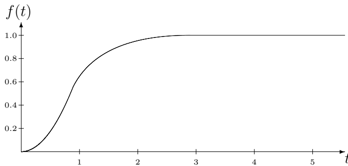
Figure 6: The function f(t) which determines the small t -behavior of either the parameter g or the update time \Delta t in the modified Necker-Zeno model.
