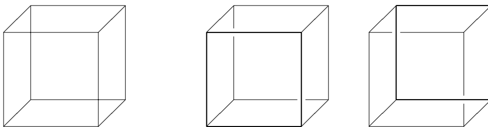
Figure 1: The Necker cube (left) and the two ways how it can be interpreted (right).
