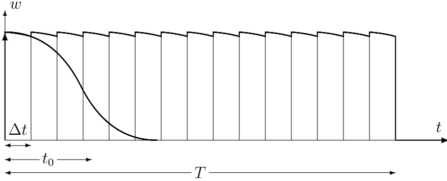
Figure 3: Time scales of the quantum Zeno effect: \Delta t is the time interval between successive observations of the system, t_0 is the time scale for the decay of the unperturbed (unobserved) system, and T is the mean decay time if the system is observed at time intervals \Delta t .
