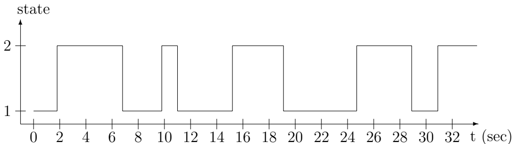
Figure 2: Schematic representation of the bistable switching between states 1 and 2 as a function of time t .
